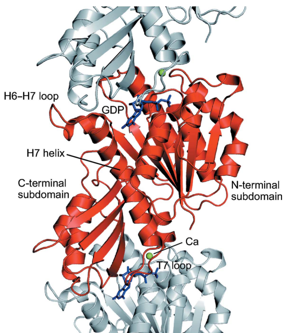
Figure 2 Crystal packing of SaFtsZf -GDP (molecule A). An asymmetric molecule and symmetry-related molecules are coloured red and grey, respectively. GDP and calcium ions are represented as blue sticks and green spheres, respectively.
