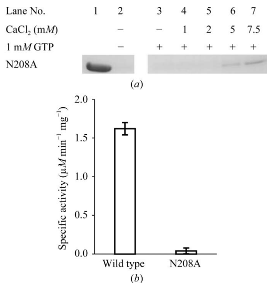
Figure 8 Sedimentation assay and GTPase activity of SaFtsZf N208A. (a) 15 \mu M SaFtsZf N208A was incubated with 1 mM GTP in the presence of varying concentrations of CaCl 2 . The samples in lanes 2–7 were precipitated by ultracentrifugation and the precipitates were analyzed by SDS–PAGE. Lane 1, 15 \mu M SaFtsZf N208A as a control; lane 2, precipitation without GTP and CaCl 2 ; lane 3, without CaCl 2 ; lane 4, 1 mM CaCl 2 ; lane 5, 2 mM CaCl 2 ; lane 6, 5 mM CaCl 2 ; lane 7, 7.5 mM CaCl 2 ; 1 mM GTP was added to the buffer in lanes 3–7. (b) GTPase specific activities of SaFtsZf and SaFtsZf N208A.
