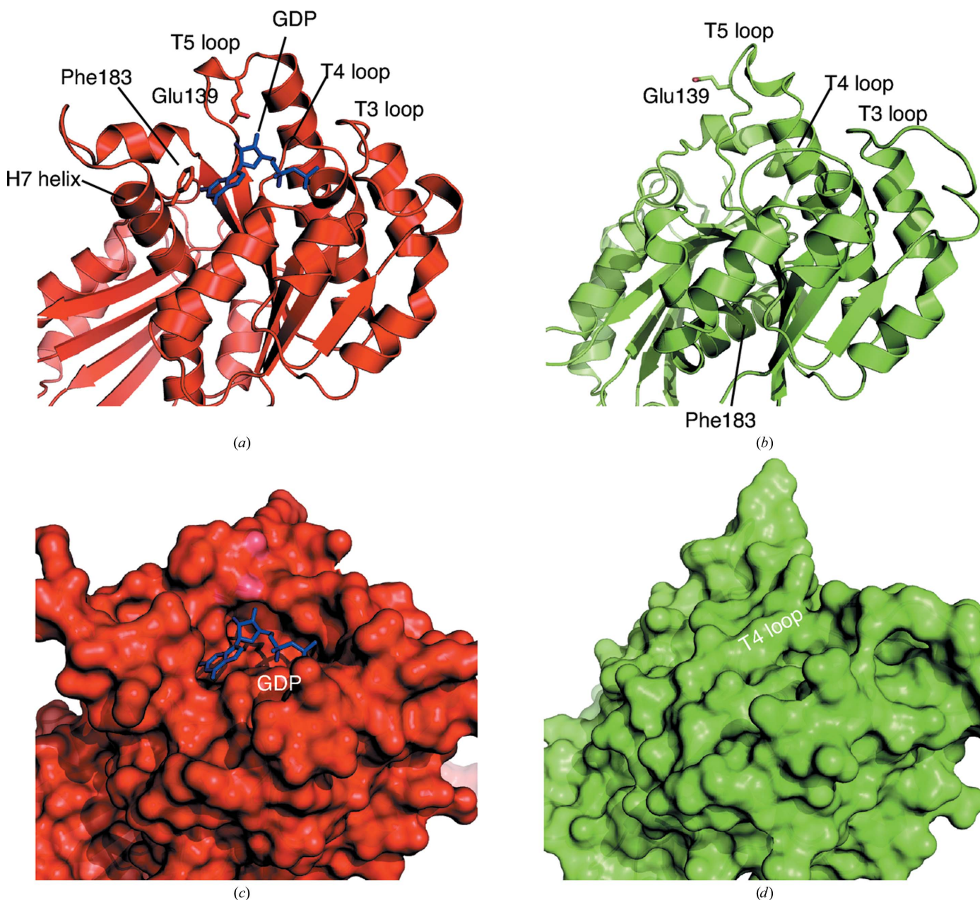
Figure 6 Structural comparison of the nucleotide-binding pockets of GDP-form (red) and apo-form (green) SaFtsZ shown in cartoon ( a , b ) and surface ( c , d ) representations. GDP bound to the GDP form is represented as blue sticks. Note that the T4 loop overlaps the GDP site in the apo form.
