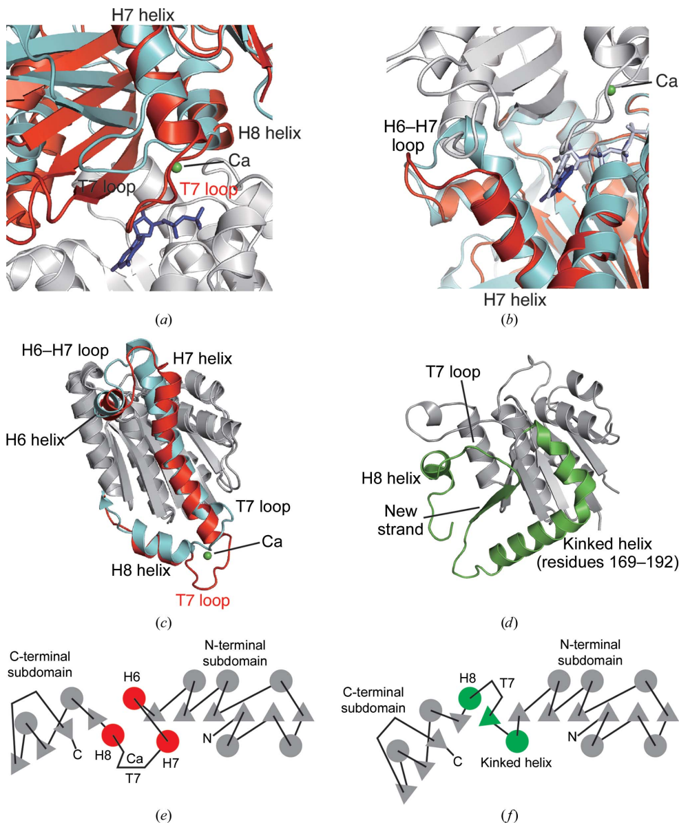
Figure 4 Structural changes in GDP-form and apo-form SaFtsZ compared with canonical FtsZ structures. ( a, b ) Molecular structure and polymer association are compared between GDP-form SaFtsZ (red) and the tilted dimer of MjFtsZ (PDB entry 1w5a; cyan). ( a ) Interactions between the T7 loop and the ‘lower’ subunit (grey) are shown. The N-terminal subdomain (residues 13–171) of the GDP form in the lower subunit was superposed on the same region of the lower subunit of MjFtsZ . GDP of SaFtsZ and the calcium ion are represented as blue sticks and a green sphere, respectively. ( b ) Conformational differences around the H6–H7 loop are shown. This figure is superposed in the same manner as in ( a ). The ‘upper’ subunit of SaFtsZ is shown in grey. GDP bound to SaFtsZ and GTP bound to MjFtsZ are shown as blue and sky-blue sticks, respectively. ( c ) Comparison of the interface region (from H6 helix to H8 helix) of the N- and C-terminal subdomains between GDP-form SaFtsZ (red) and MjFtsZ (cyan) showing that the H7 helix and T7 loop of SaFtsZ are downshifted by about one helical pitch. The view is looking down from the C-terminal subdomain (residues 223–316) towards the N-terminal subdomain (residues 12–166) after superposition of the N-terminal subdomains of SaFtsZ and MjFtsZ (the N-terminal extra helix is omitted). The N-terminal subdomains of both structures are coloured grey and the C-terminal subdomain is not shown for clarity. ( d ) The conformation of the apo form is shown in the same manner as in ( c ). The interface region (corresponding to the region from H6 helix to H8 helix of the GDP form) is coloured green. ( e, f ) Topological diagrams of secondary structure are shown for ( e ) the GDP form and ( f ) the apo form. Circles and triangles indicate \alpha -helices and \beta -strands, respectively. The interface region between subdomains of the GDP form and the apo form are coloured red and green, respectively.
